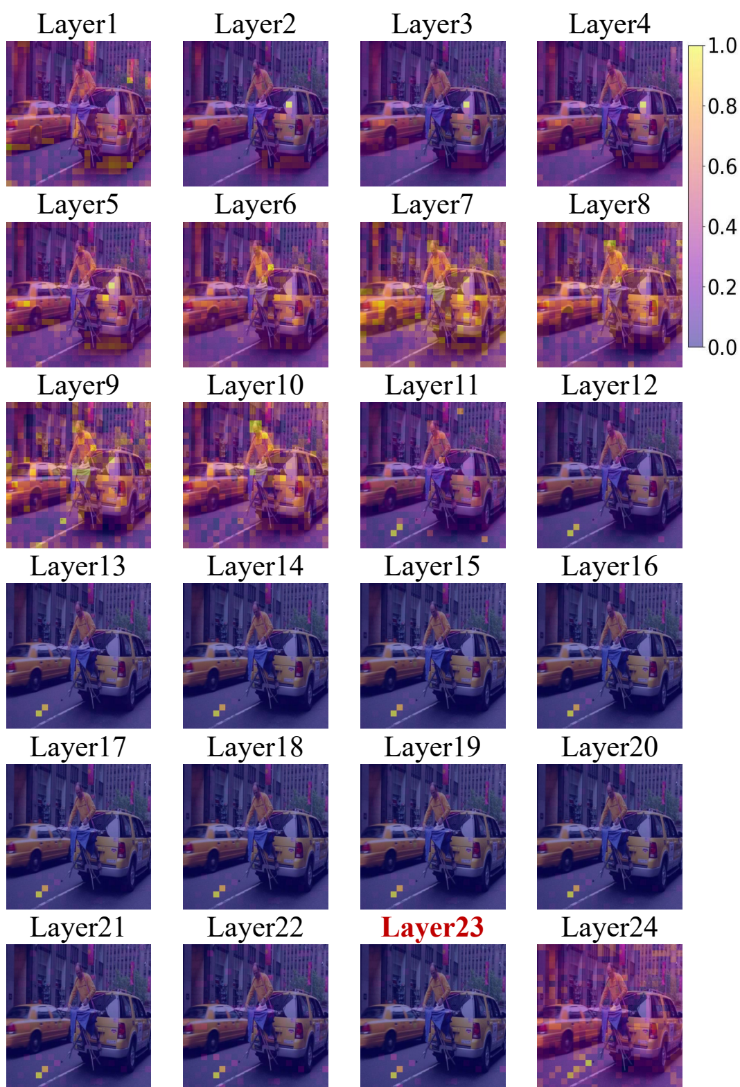
Figure 13. Visualization of Attention Distribution Change
