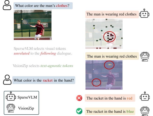
Figure 7. Example comparison of VisionZip and previous text-relevant method in multi-turn conversation
