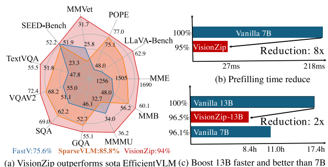
Figure 1. VisionZip Performance and Efficiency. (a) Our VisionZip significantly outperforms the current SOTA EfficientVLM model, like FastV, SparseVLM, achieving nearly 95% of the performance with only 10% of the tokens across 11 benchmarks on LLaVA-1.5. (b) VisionZip could reduce 8× prefilling time for LLaVA-NeXT 7B. (c) VisionZip reduces GPU inference time by 2× across 11 benchmarks, enabling the LLaVA-NeXT 13B model to infer faster than the 7B model while achieving better results.
