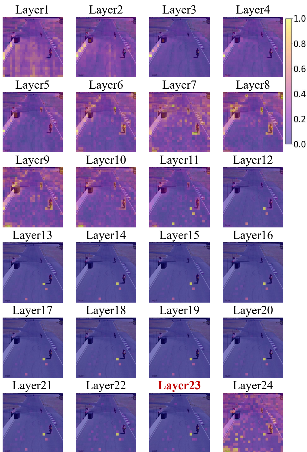
Figure 12. Visualization of Attention Distribution Change
